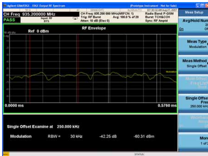
EDGE ORFS Result - Modulation with Single-Offset (Examine)
