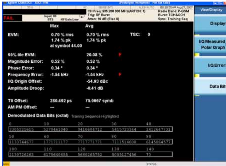
Figure 3-7 EDGE EVM Result - Data Bits View
