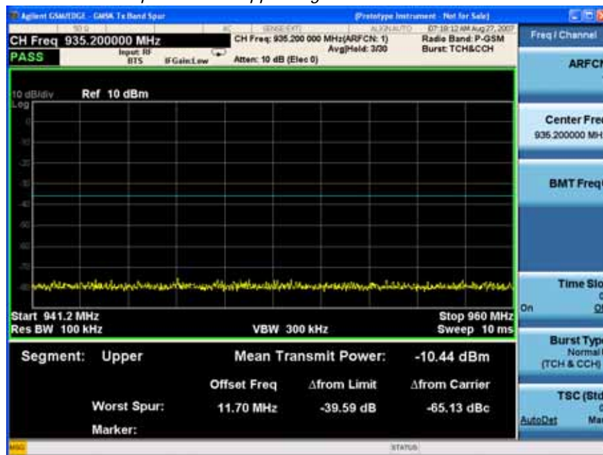
Figure 2-20 GMSK Tx Band Spur Result - Upper Segment
