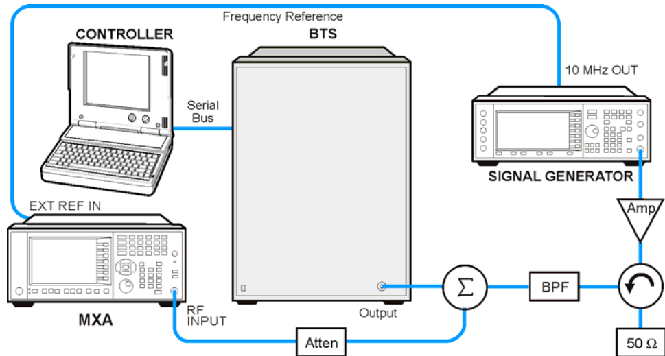
Figure 2-19 GMSK Transmitter Band Spurious Measurement System
