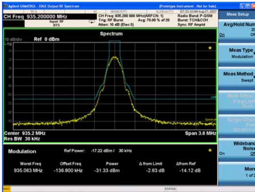
EDGE ORFS Result - Modulation Sweep Spectrum
