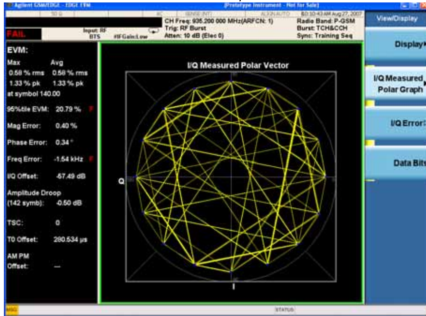
Figure 3-5 EDGE EVM Result- IQ Measured Polar Graph
