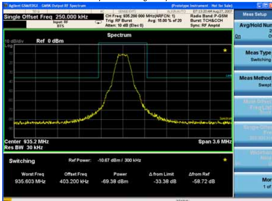
GMSK ORFS Result - Example Switching Swept View
