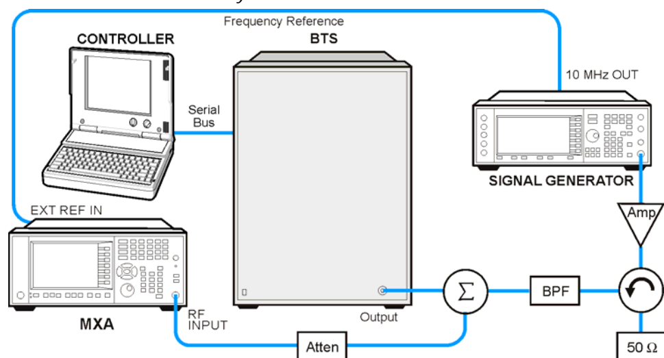
GMSK ORFS Measurement System
