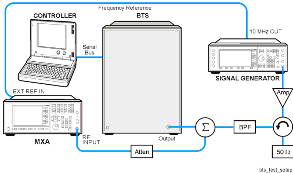
Figure 2-7 GMSK Phase and Frequency Measurement System
