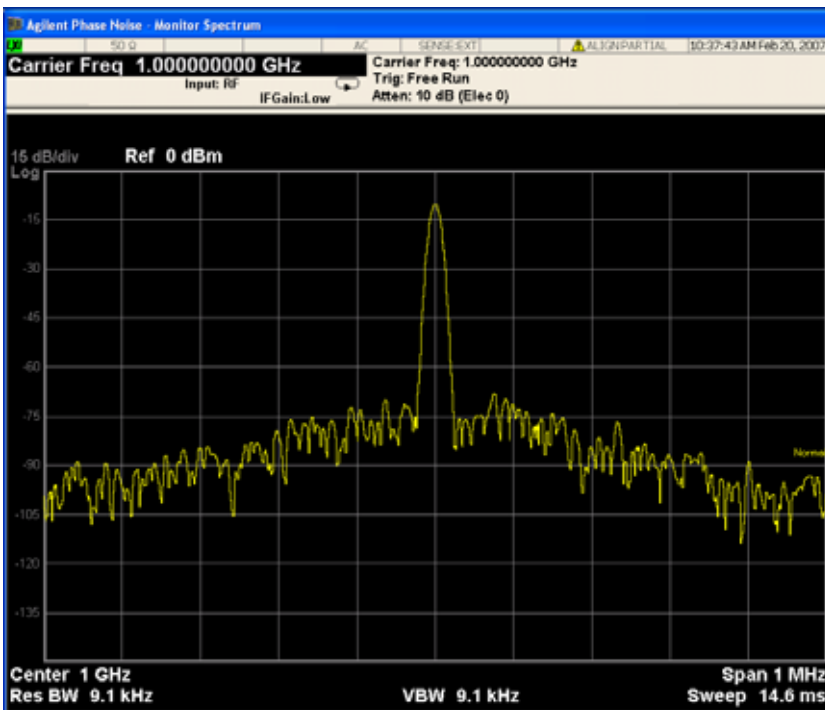
Figure 2-40 Monitor Spectrum Measurement - Spectrum and I/Q Waveform (Default View)
