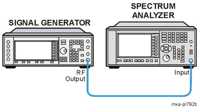
Figure 2-39 Monitor Spectrum Measurement
